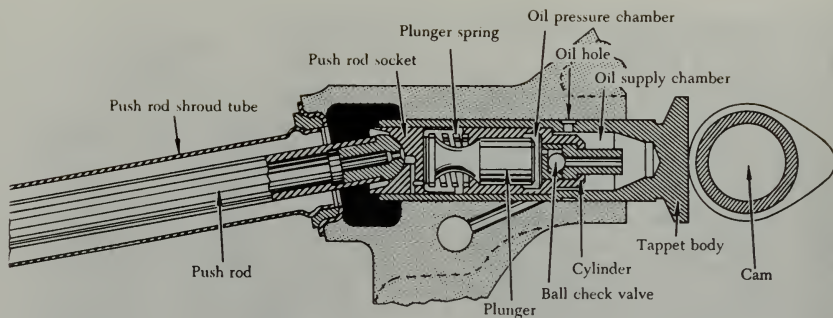
FIGURE 1-22. Hydraulic valve tappets.
